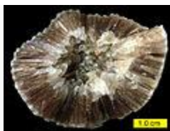
Calcite crystals inside a test of the cystoid Echinospaerites aurantium (Middle Ordovician , northeastern Estonia ).
