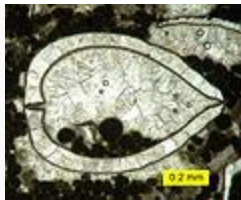
Thin section view of calcite crystals inside a recrystallized bivalve shell in a biopel sparite.
